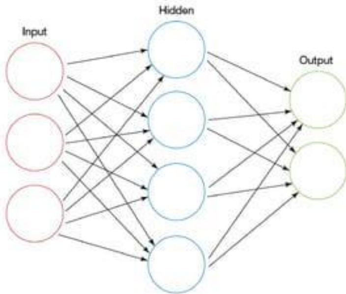
Multi-layer perceptron
